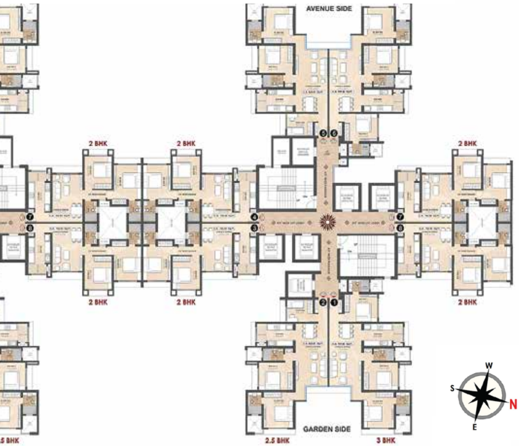
TOWER C TYPICAL FLOOR PLAN
